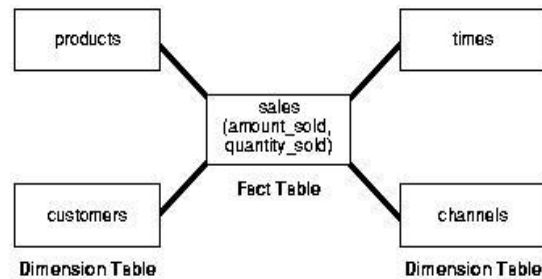
Figure 3.1 Star Schema
