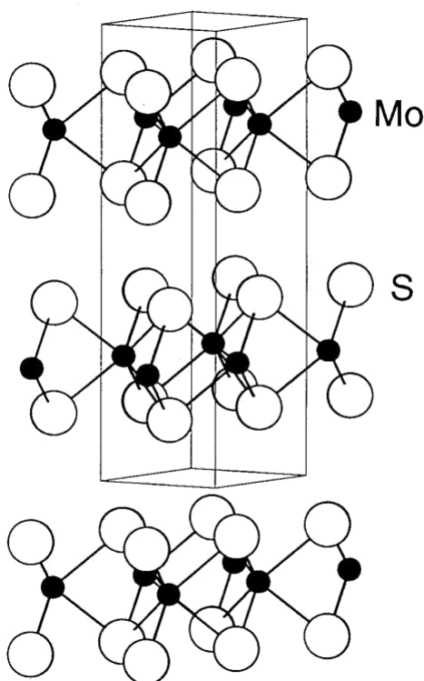
Fig. 4.19 Structure of MoS_2 .
