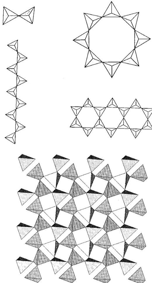
Fig. 4.9 Bridging modes of the SiO 4 tetrahedra.
