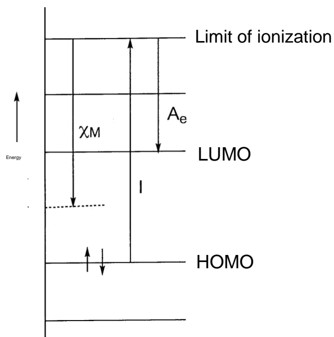
Fig. 2.14 Mulliken electronegativity.
