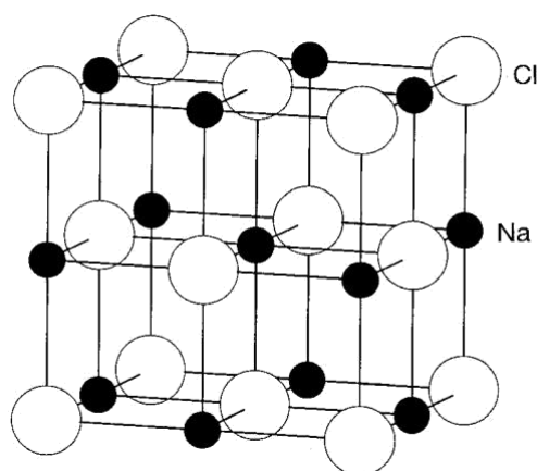
Fig. 2.7 Rock-salt structure.
