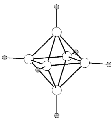
(a) closo - [B_6H_6]^{2-}
