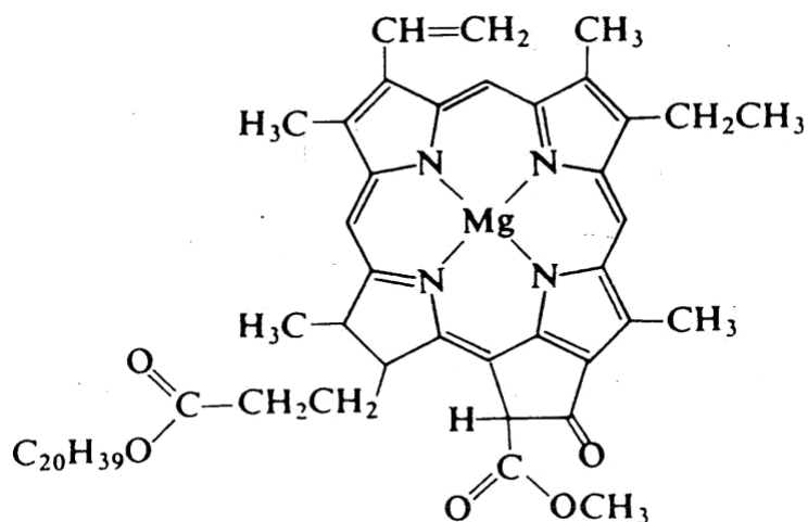
Figure 8.3 Chlorophyll a .
