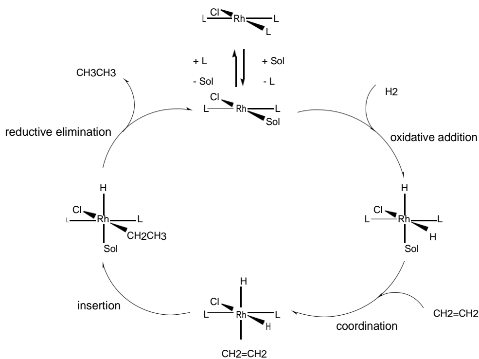
Figure 8.1 Catalytic cycle of ethylene hydrogenation by the Wilkinson catalyst.
