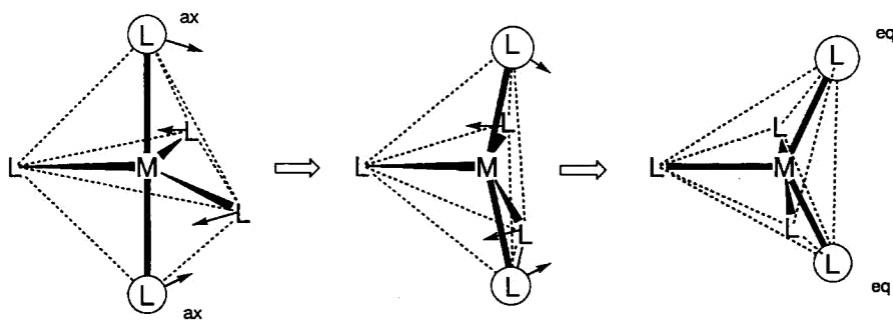
Fig. 6.2 Berry's pseudorotation.
