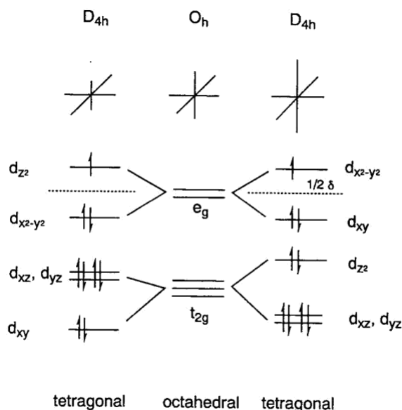
Fig. 6.8 Jahn-Teller splitting in a Cu 2+ ion.
