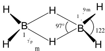
Fig. 4.2 Structure of diborane.
