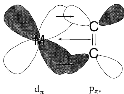
Fig. 6.17 Back-donation in olefin complexes.
