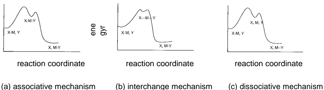
Fig. 6.26 The stability of the intermediate of ligand substitution.
