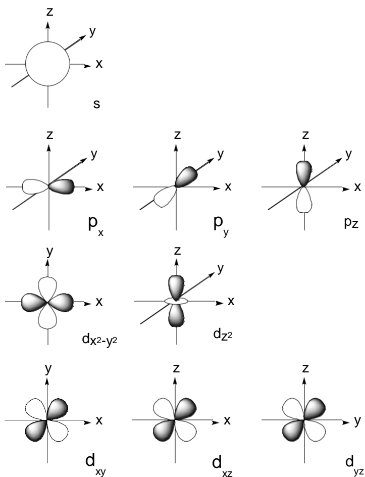
Fig. 1.1 Shapes of s , p , and d orbitals.
