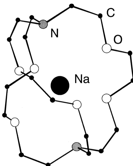
Fig. 5.1 Structure of Na(crypt).
