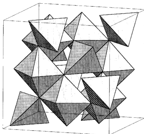
Fig. 4.15 Spinel structure.
