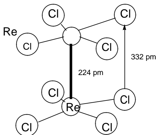
Fig. 6.21 Structure of \text{Re}_2\text{Cl}_8^{2-} .
