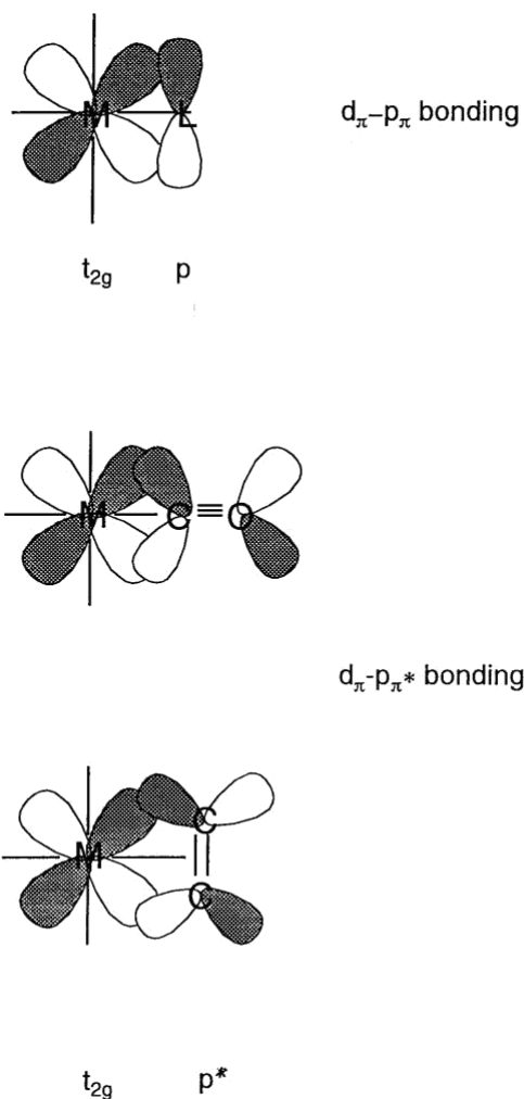
Fig. 6.11 The relation between the metal and ligand orbitals in formation of a \pi bond.
