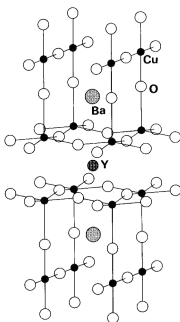
Figure 8.4 Structure of YBa 2 Cu 3 O 7-x .
