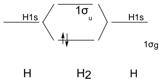
Fig. 2.18 The molecular orbitals of H_2 . The arrows indicate the electron spins.
