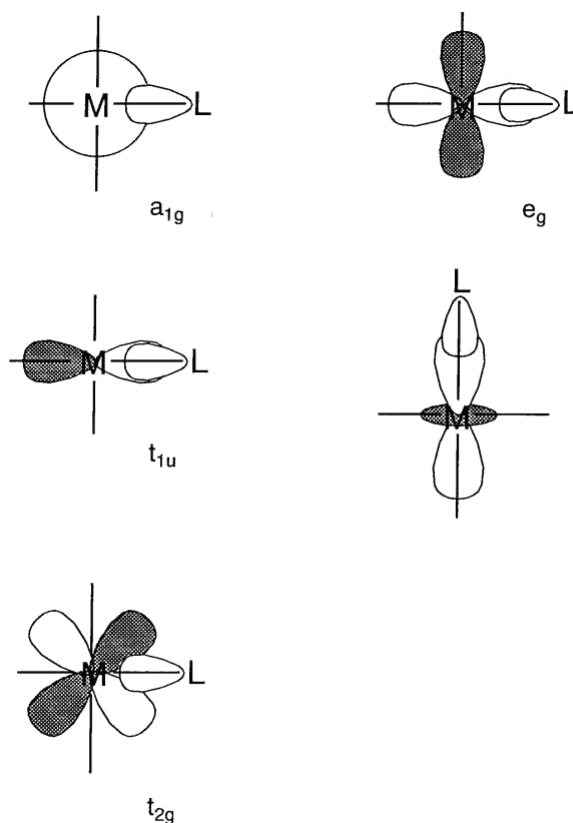
Fig. 6.9 The relation between the metal and ligand orbitals during formation of \sigma bonds.
